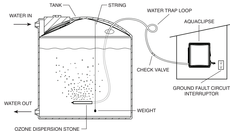
Figure 1: Recommended Installation
