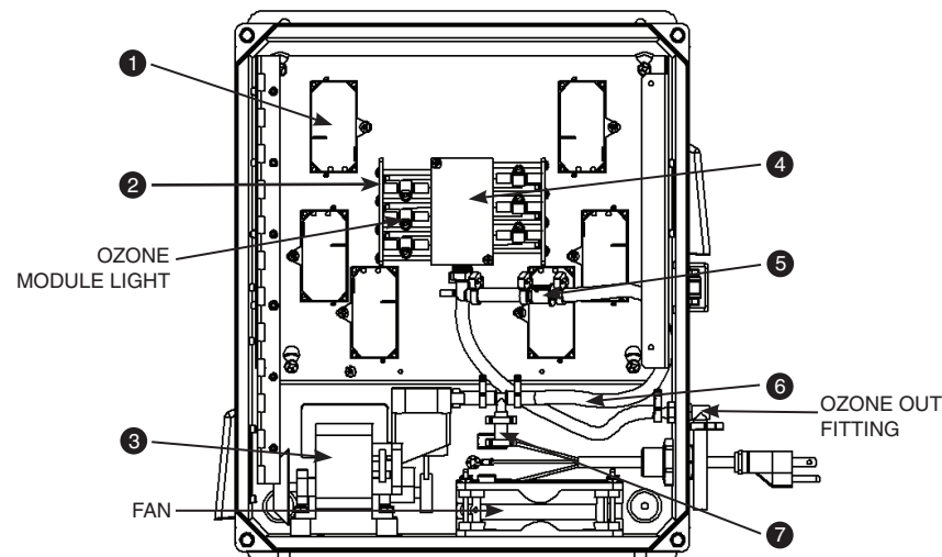
Figure 2: ZO-400 Internal View
