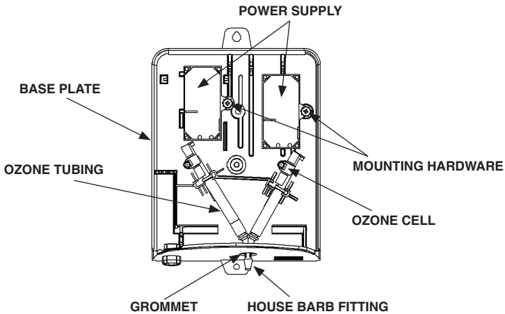
Figure 6: Internal Component Locations
