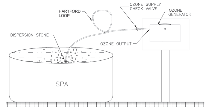
Figure 2. Standard Installation Diagram
