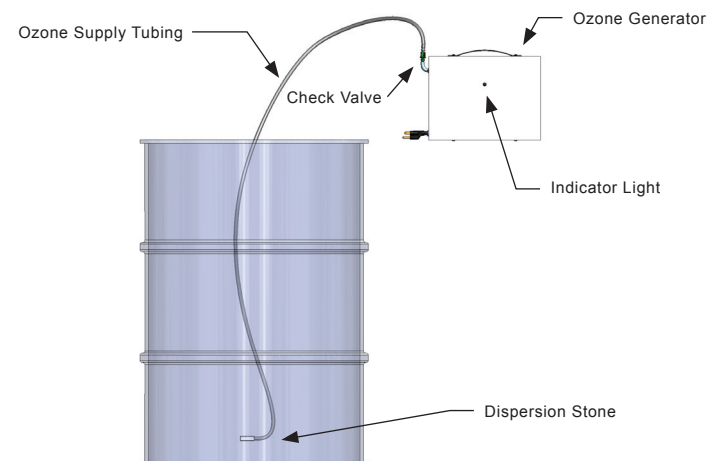
Figure 1. Example Installation Diagram
