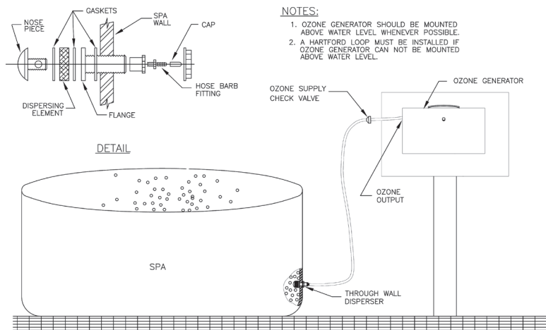
Figure 3. Thru-Wall Disperser Installation Diagram
