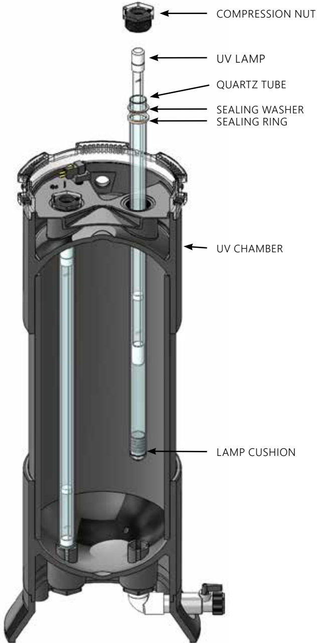
Figure 4: System Electromechanical Overview
